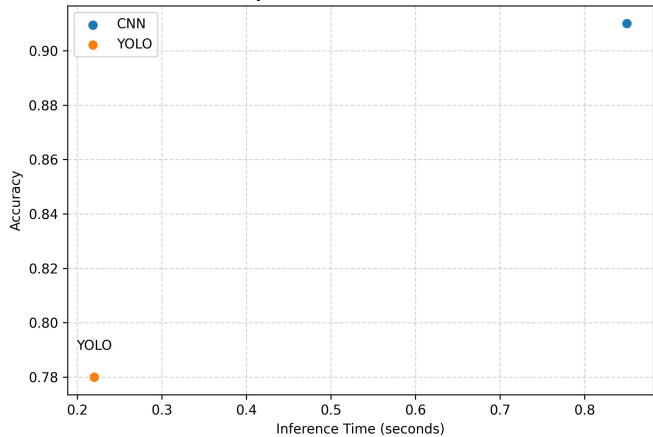
Accuracy vs Inference Time: CNN vs YOLO
