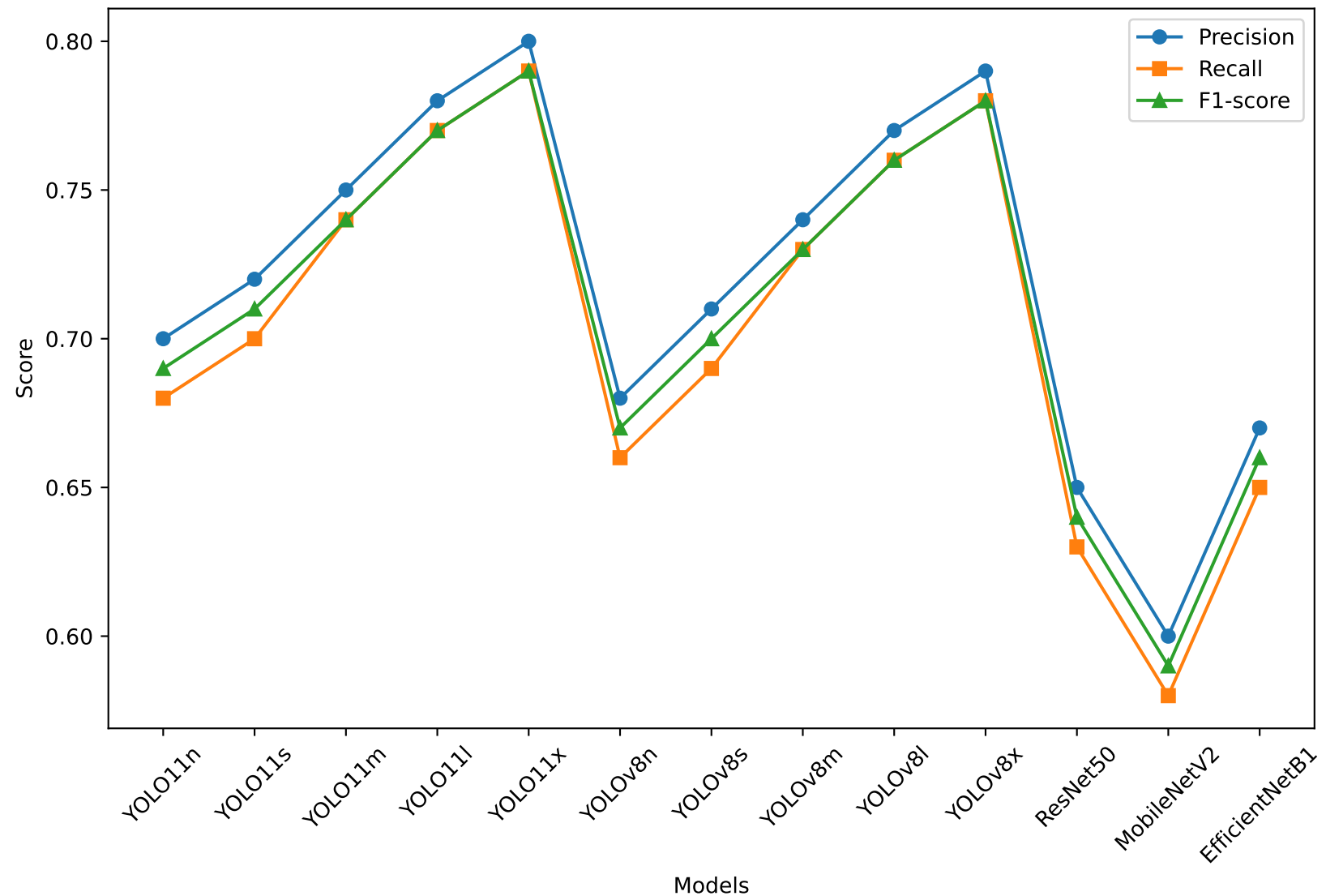
Precision, Recall, F1-score (Line)
