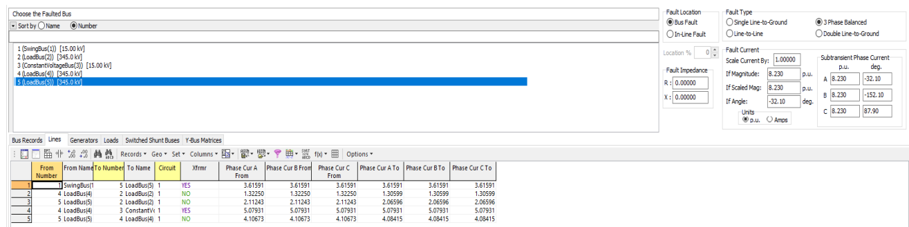
Fig: Fault Currents in Bus-5
