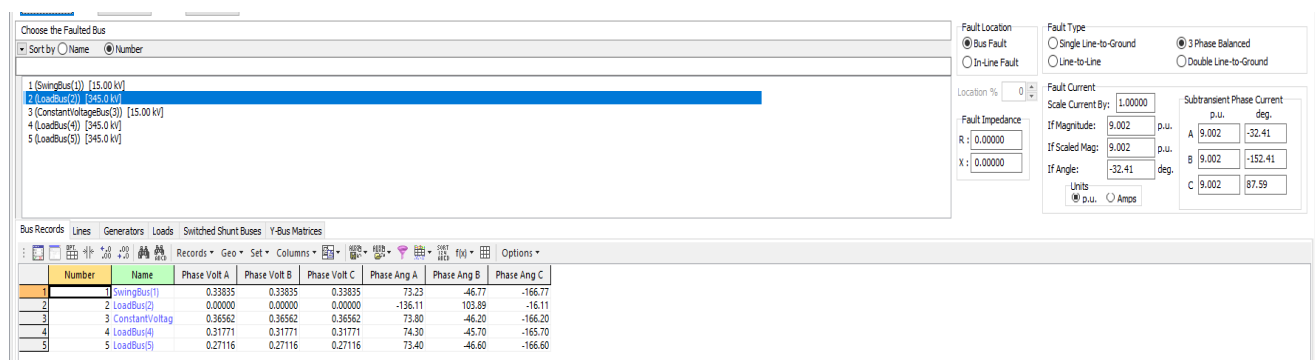
Fig: Fault Voltages in Bus-2
