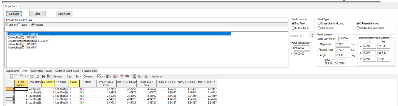
Fig: Fault Currents in Bus-1
