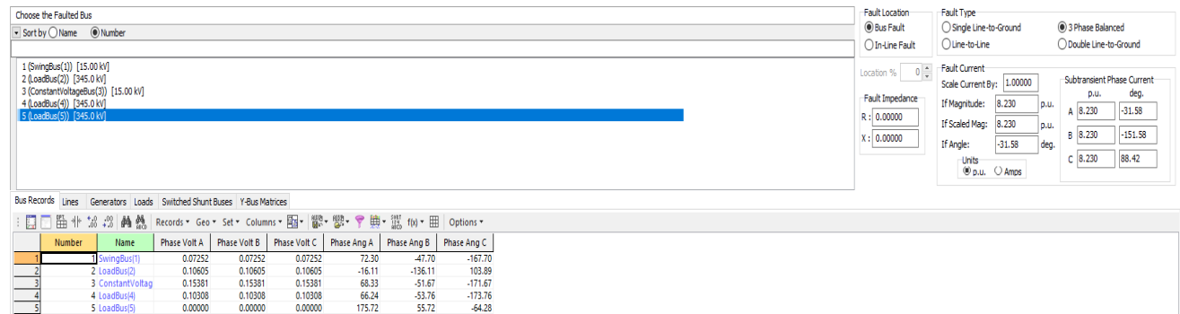
Fig: Fault Voltages in Bus-5
