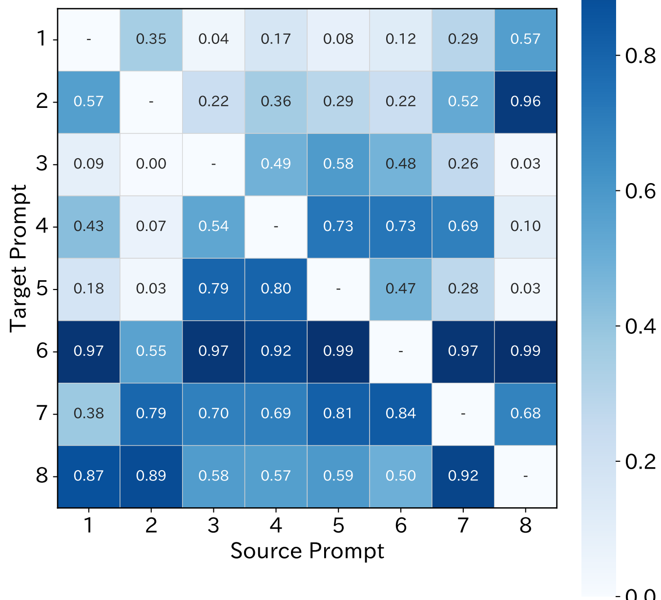
(a) Selection Rate
