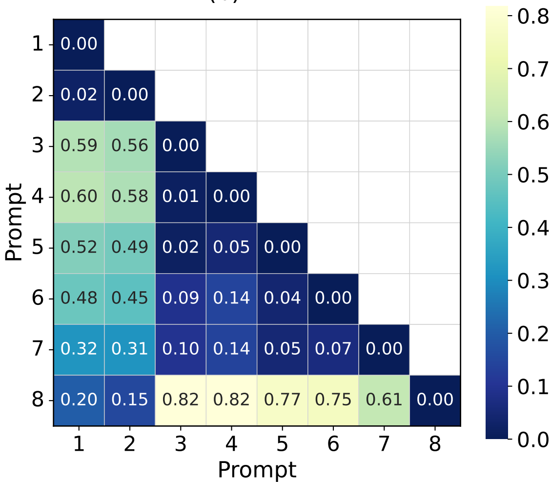
(b) MMD
