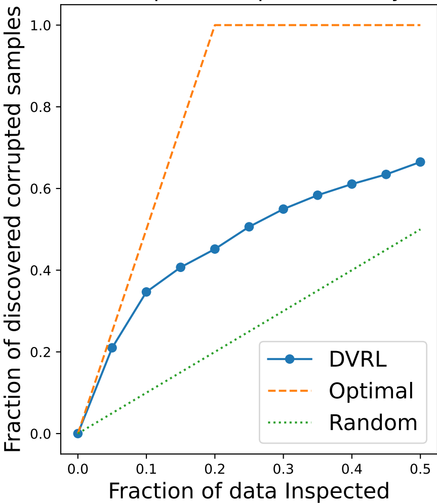
Corrupted Sample Discovery
