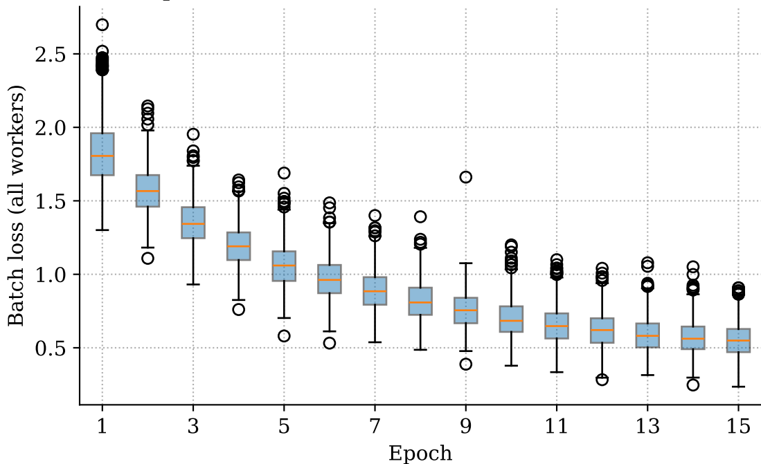
Per-epoch batch loss distribution across all workers
