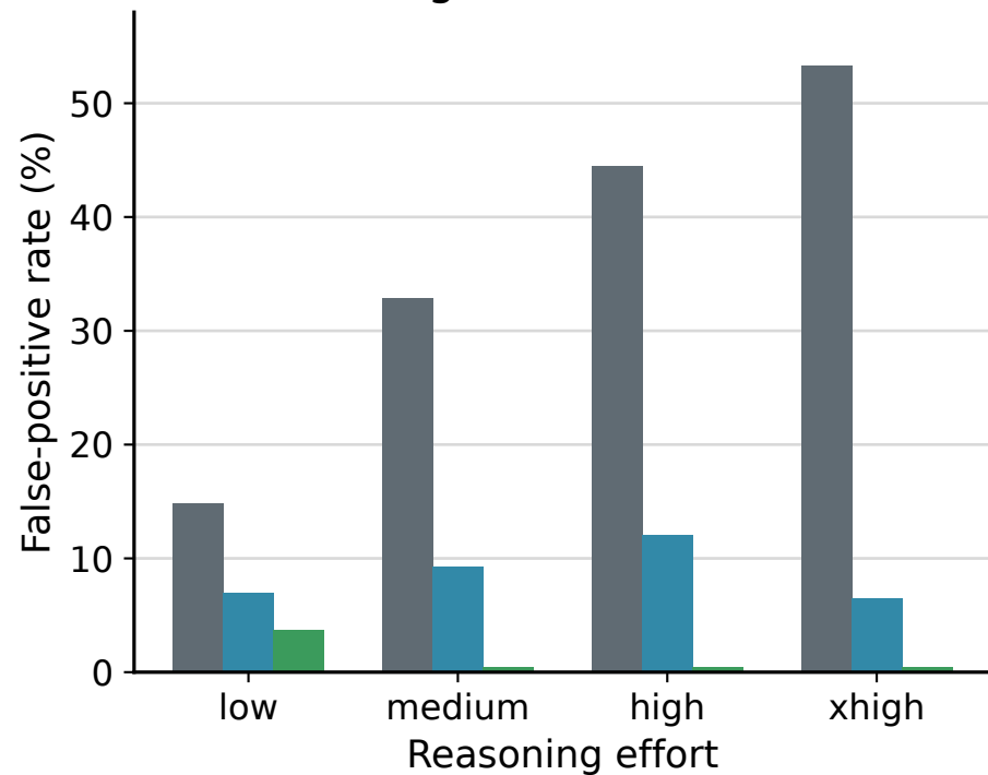
(a) Overcalling absent traces
