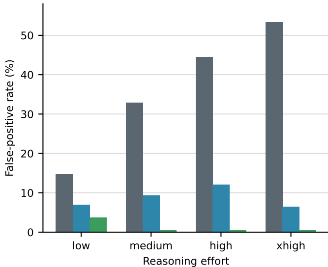
(a) Overcalling absent traces
