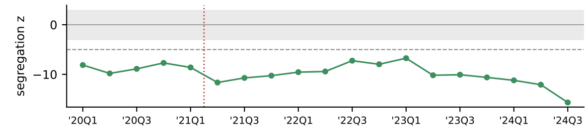
DD control (five analysis subreddits), union lens, B = 4
