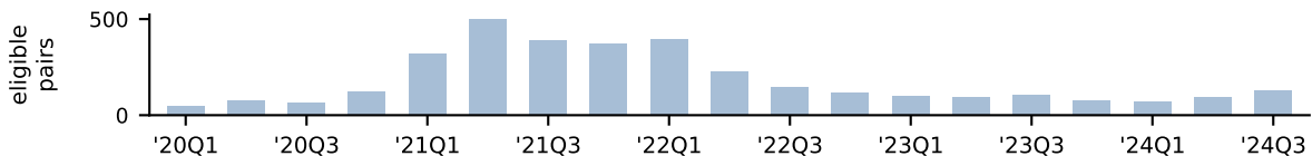
DD control (five analysis subreddits), union lens, B = 4
