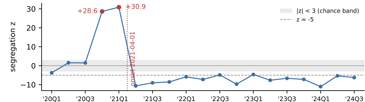
r/wallstreetbets (treatment), union lens, B = 4
