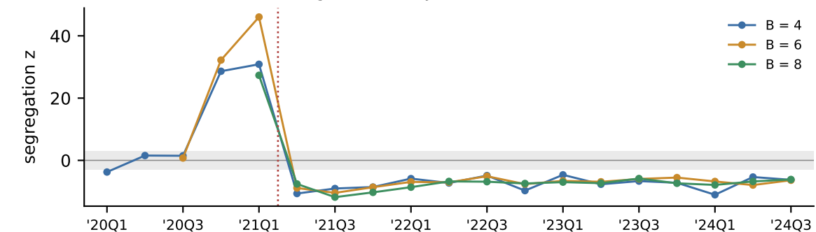
window-length sensitivity: WSB union z at B = 4 / 6 / 8
