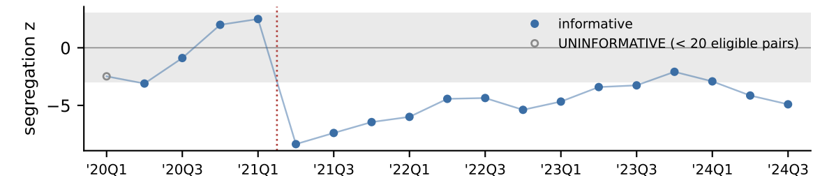
lens sensitivity: WSB cashtag z, B = 4
