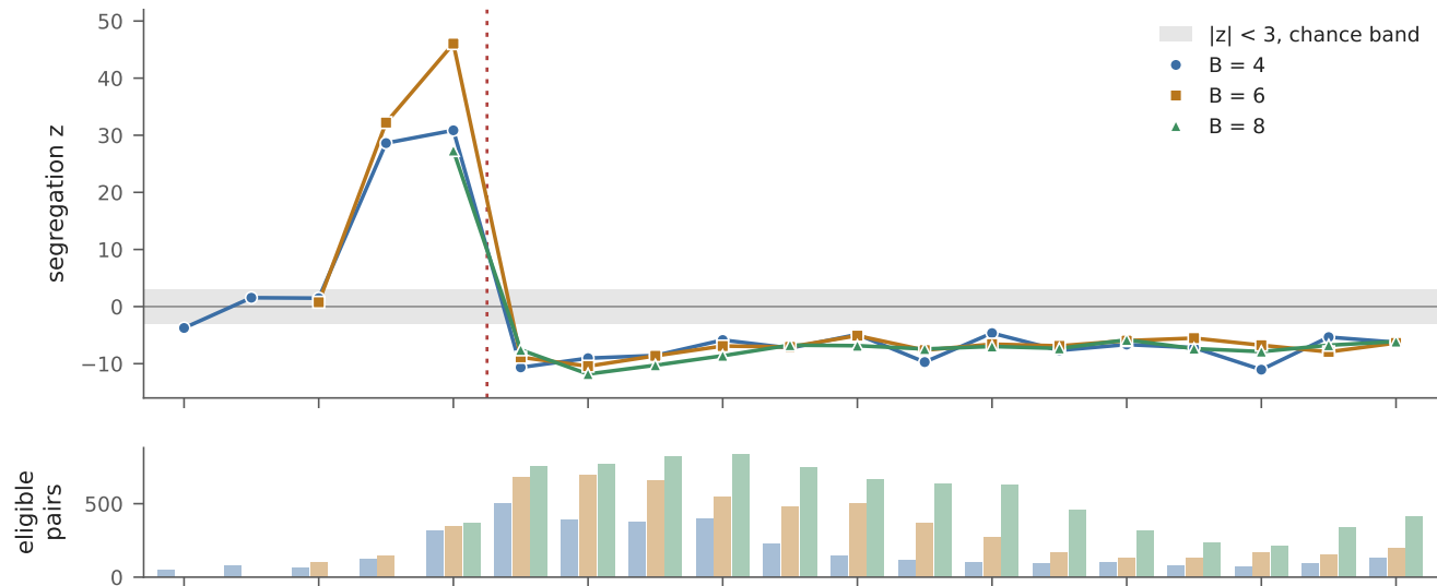
a window-length sensitivity, r/\text{wallstreetbets} , union lens
