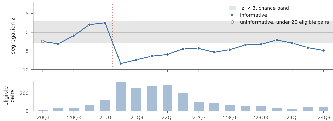
b lens sensitivity, r/\text{wallstreetbets} , cashtag lens
