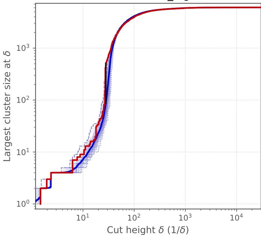
Cluster sizes across hierarchy cuts for STRING basal_logFC
