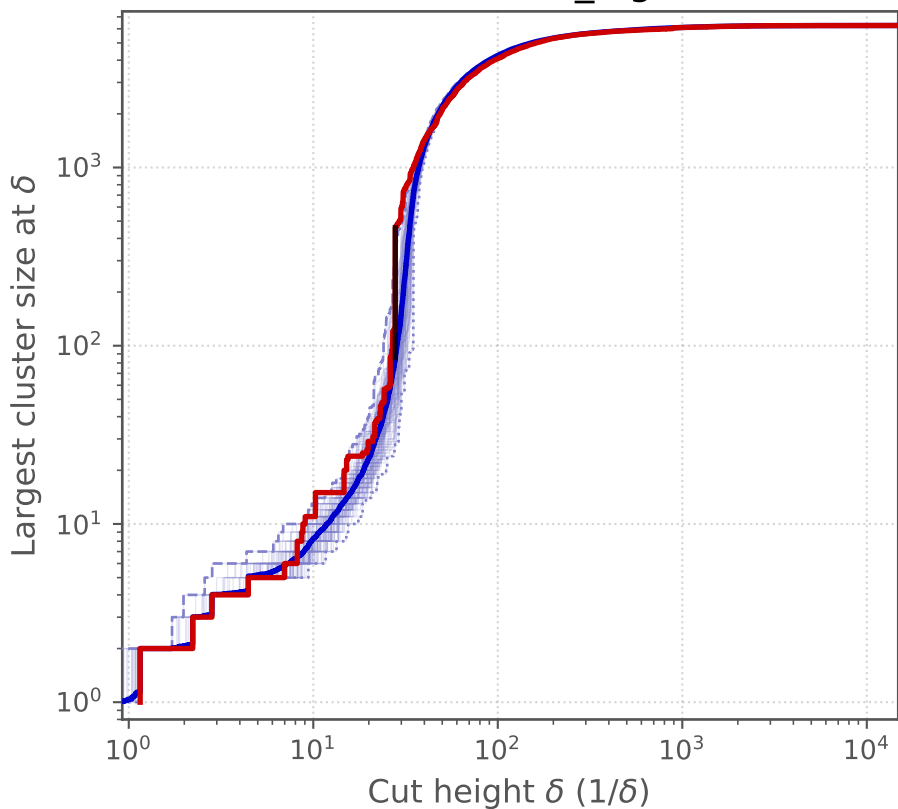
Cluster sizes across hierarchy cuts for STRING lumB_logFC
