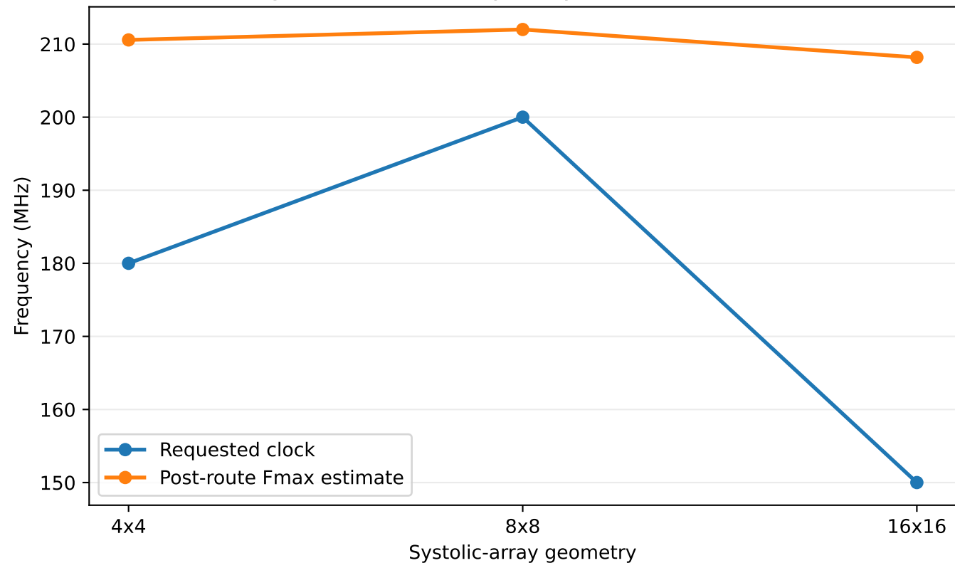
Timing Closure Across Physically Validated Accelerators
