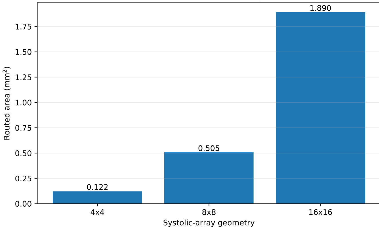
Post-Route Area Scaling
