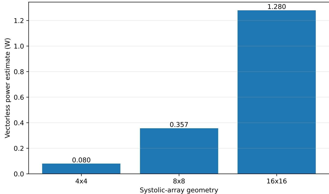
Post-Route Vectorless Power Scaling
