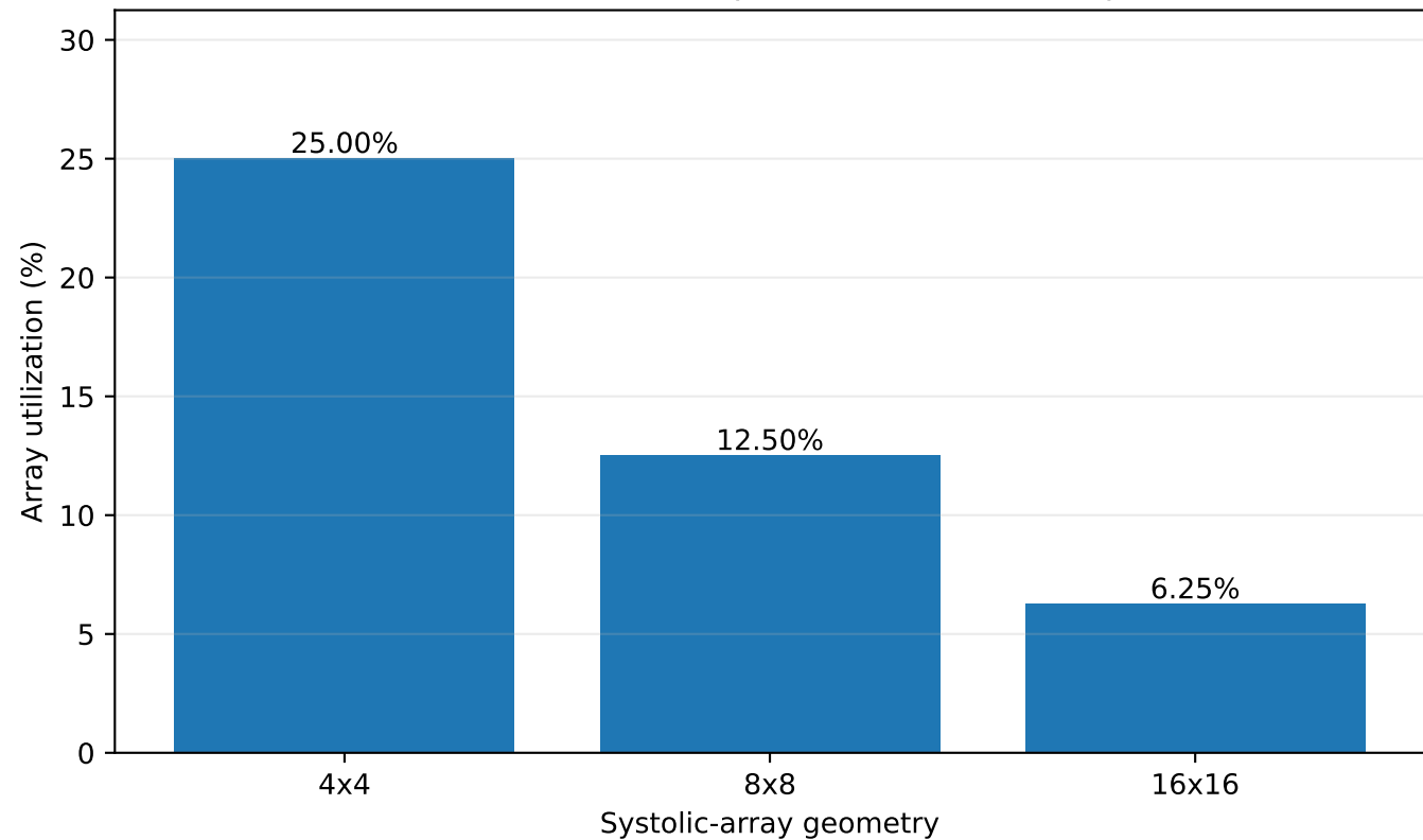
LLM Token Decode: Spatial Utilization Collapse
