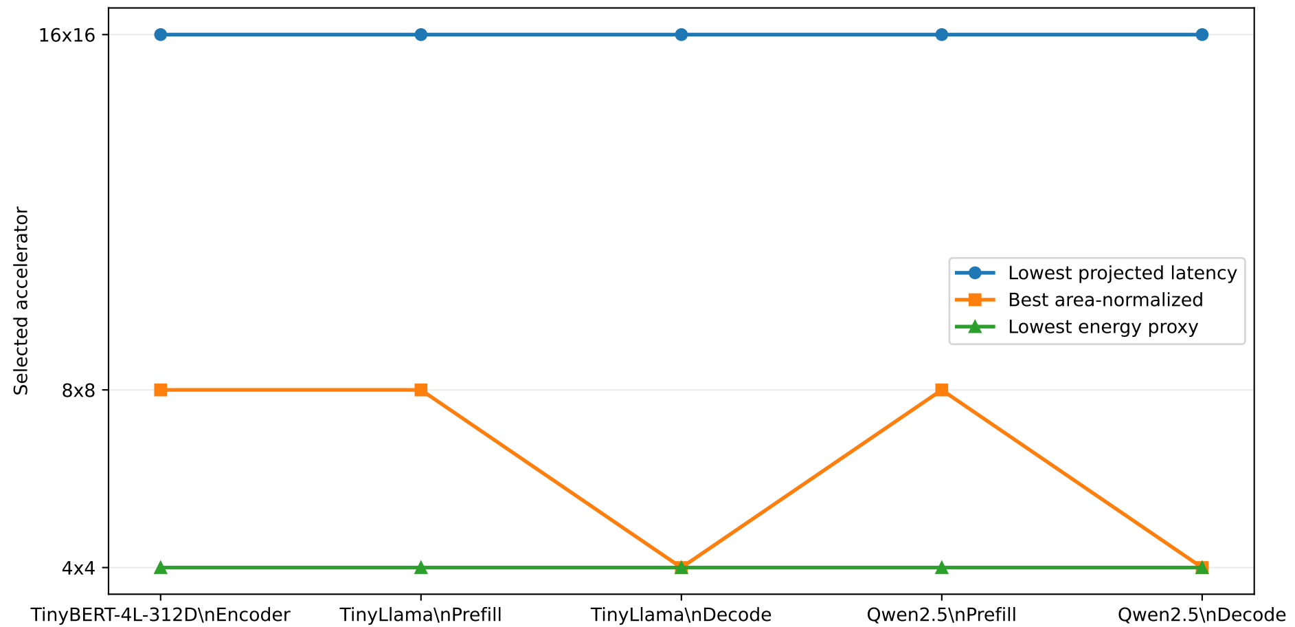
AccelClosure Workload-Aware Hardware Selection
