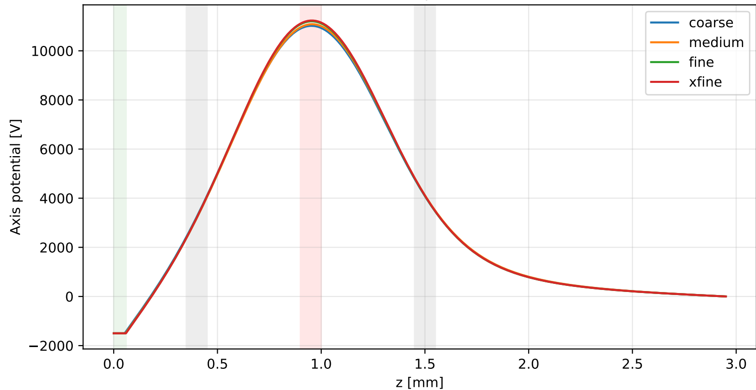
Mesh refinement: axis potential (ref = xfine)
