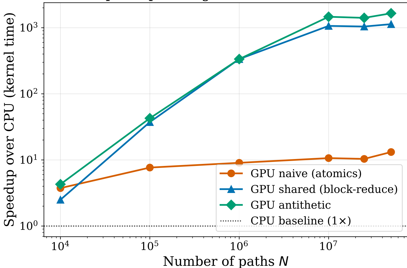
GPU speedup vs single-threaded CPU baseline
