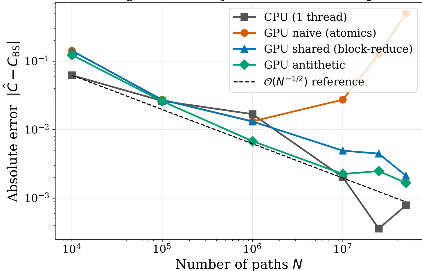
Convergence to analytical Black-Scholes price
