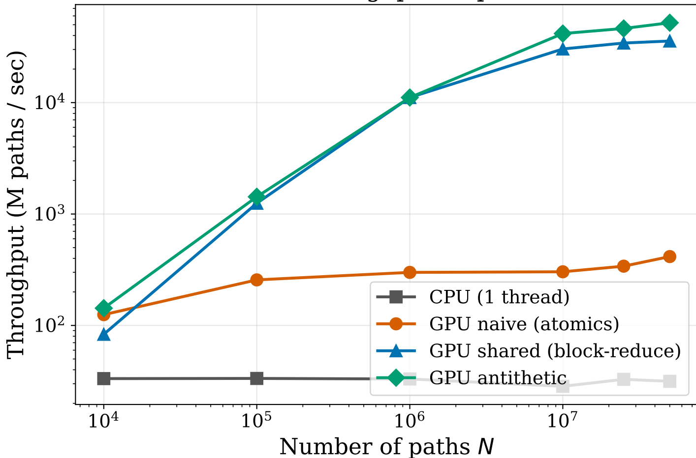
Monte Carlo throughput vs problem size
