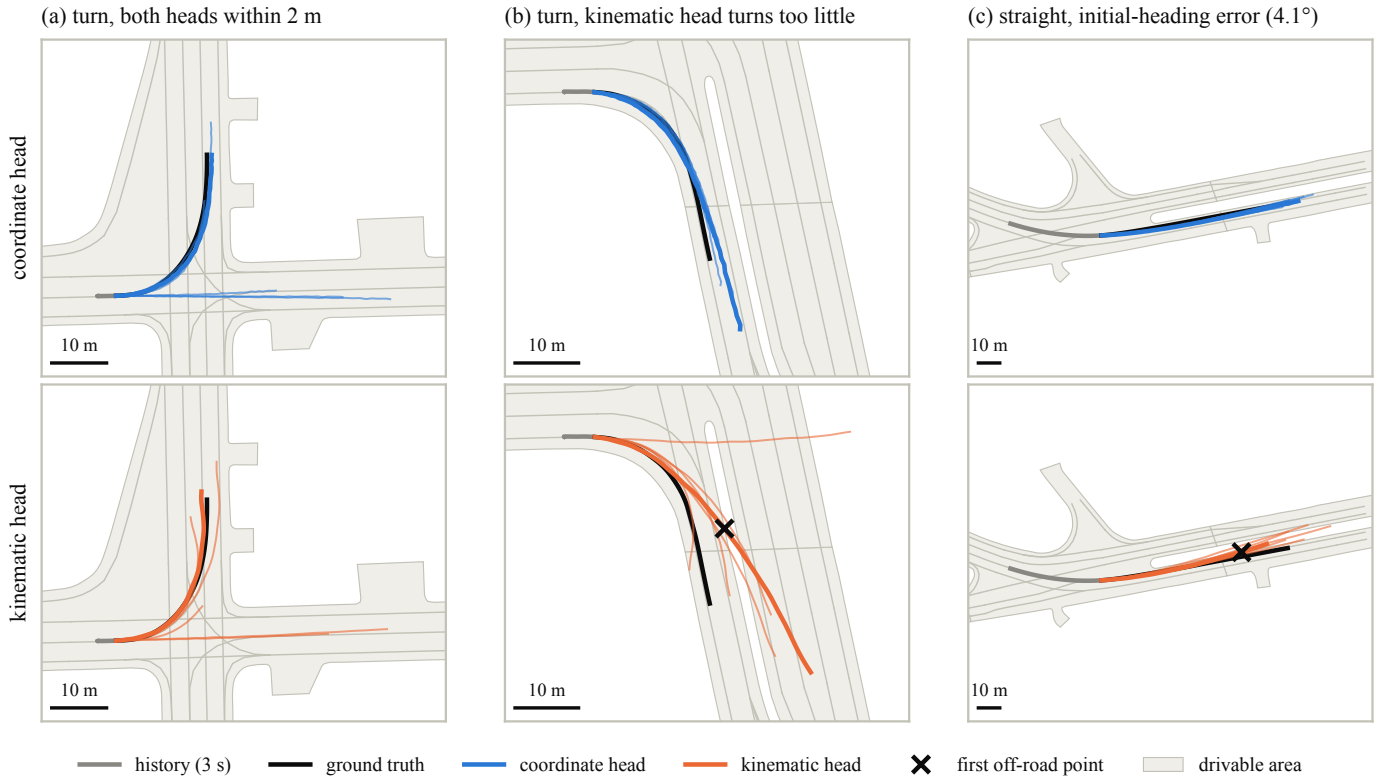
Fig. 3. Dev scenes, each drawn at random from the scenes that meet its condition. Thick lines are the most probable modes. (a) A turn in which both heads’ most probable modes end within 2 m (one of 3). (b) A turn in which the kinematic head’s most probable mode turns the right way but only 25–75% as far, and leaves the road while the coordinate head’s stays on it (one of 19). (c) A straight road on which the kinematic head starts 4.1° off the ground truth’s direction and keeps that heading across the median (one of 21).
