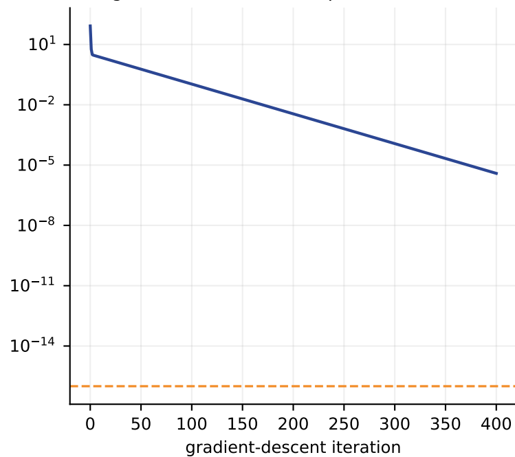
Descending to the answer least squares wrote down at once
