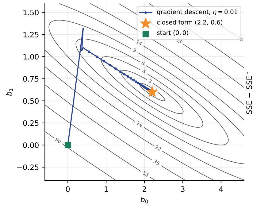
SSE( b_0, b_1 ) is a bowl with exactly one bottom
