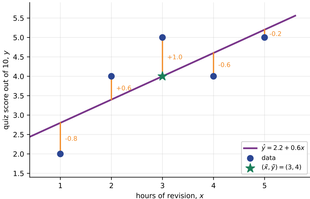
The least-squares line, and the five residuals it leaves (SSE = 2.40)
