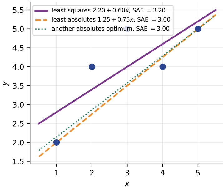
Two different lines, the same absolute error
