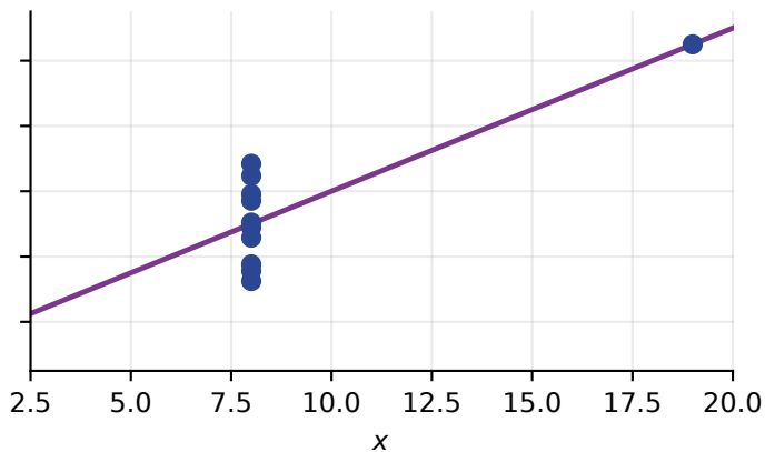
IV: R^2 = 0.6667 --- one point sets the slope
