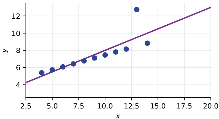
III: R^2 = 0.6663 --- a straight line and one outlier
