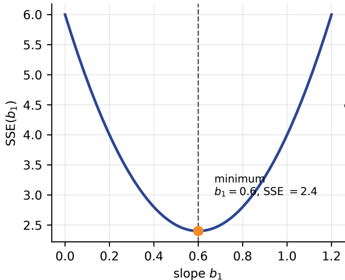
Sum of squared errors
