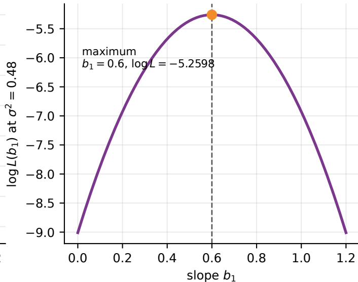
Gaussian log-likelihood
