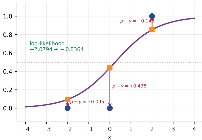
after one step, \eta = 0.5 : w = (-0.25, 1.0)
