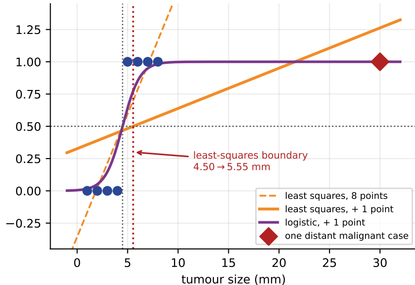
one distant point moves the least-squares boundary
