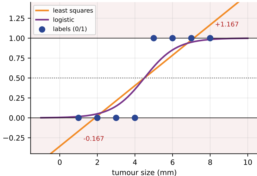
a straight line leaves [0, 1]
