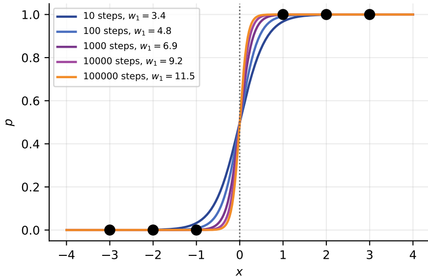
nothing stops it: the curve becomes a step
