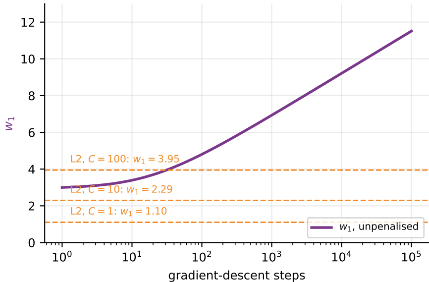
w_1 grows without bound; L2 stops it
