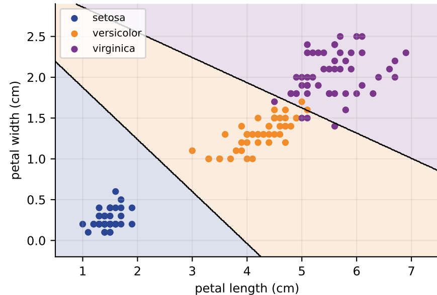
softmax: three linear scores, one normalisation
