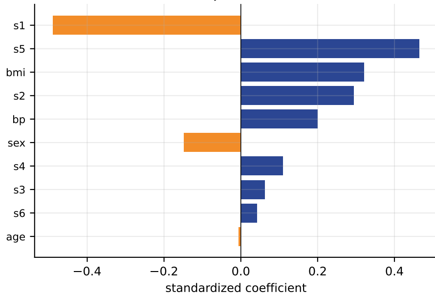
standardized \beta_j^* = b_j s_j / s_y (unit-free)
