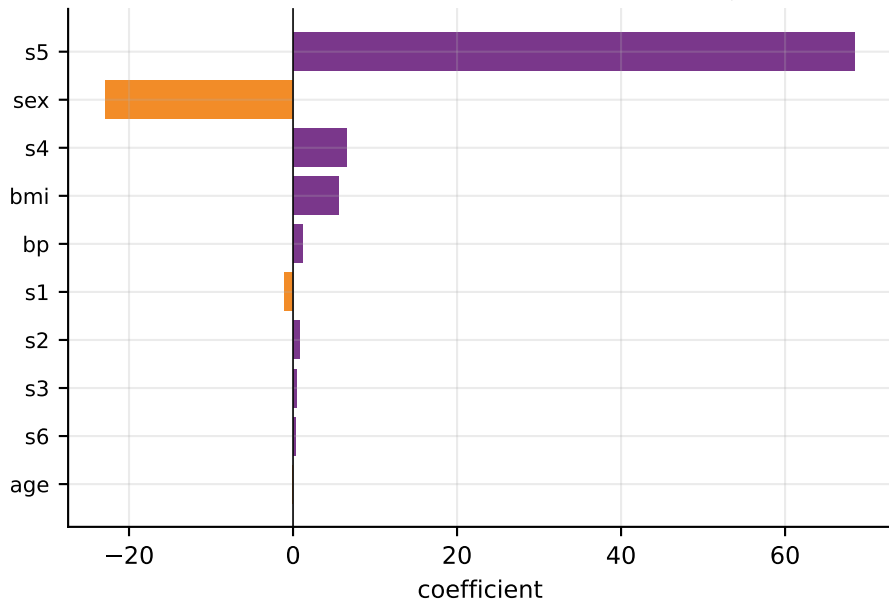
raw coefficients (units of y per unit of x_j )
