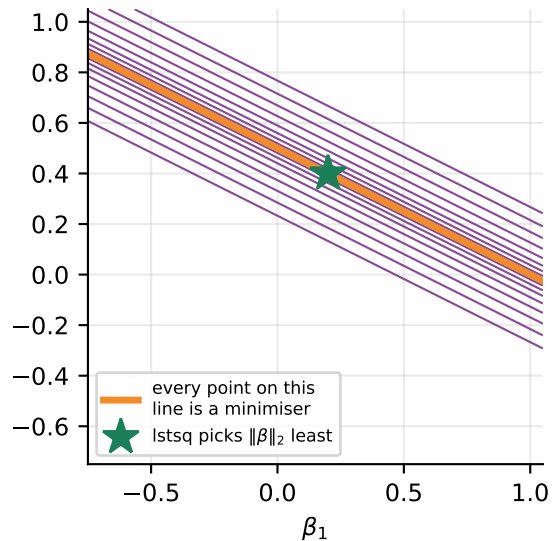
\lambda = 0 : contours are parallel LINES eigenvalues (0, 70)
