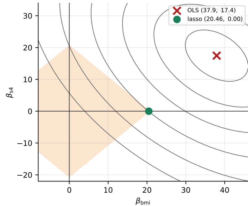
\|\beta\|_1 \leq t : a diamond, corners on the axes
