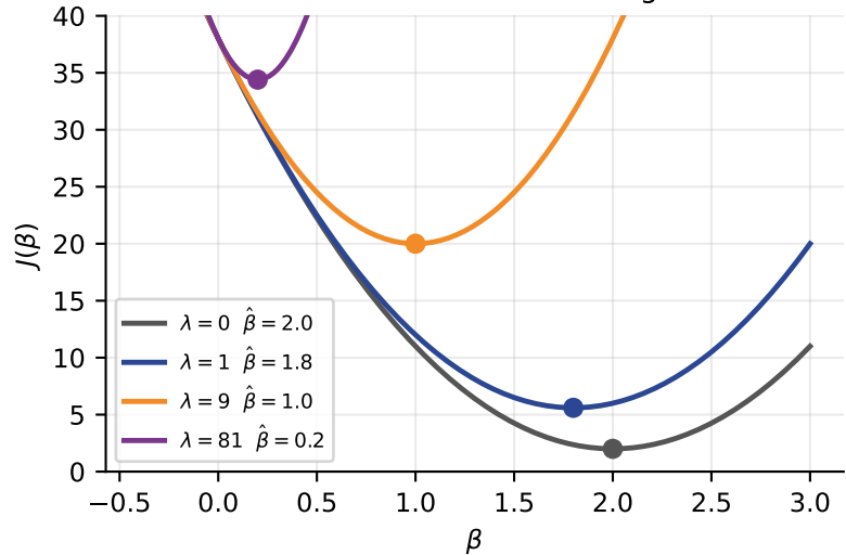
the minimum slides left as \lambda grows
