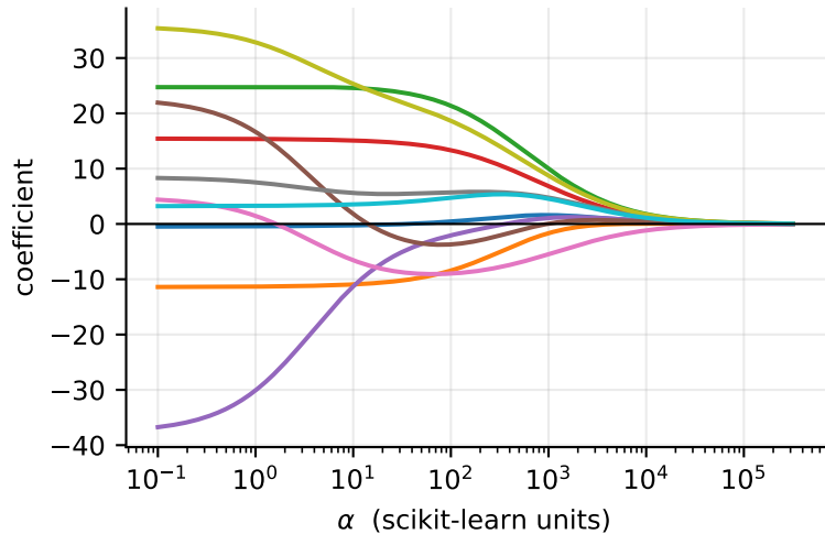
ridge: 10 curves decay smoothly, none reaches 0
