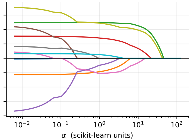
lasso: curves hit exactly 0, one at a time
