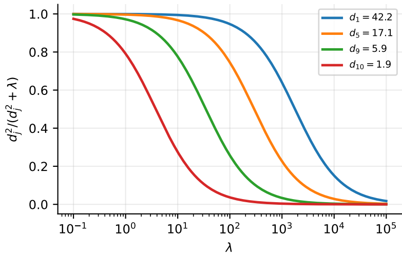
diabetes: narrow directions are crushed first
