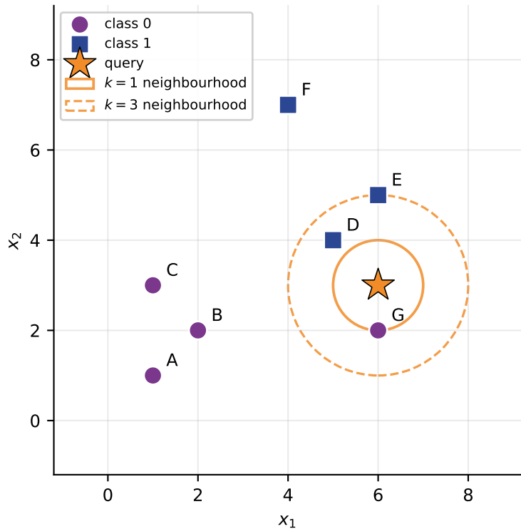
q_2 = (6, 3) : 1-NN says class 0, 3-NN says class 1
