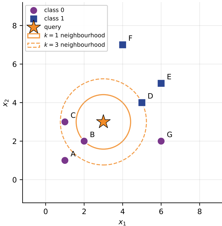
q_1 = (3, 3) : 1-NN is B, class 0
