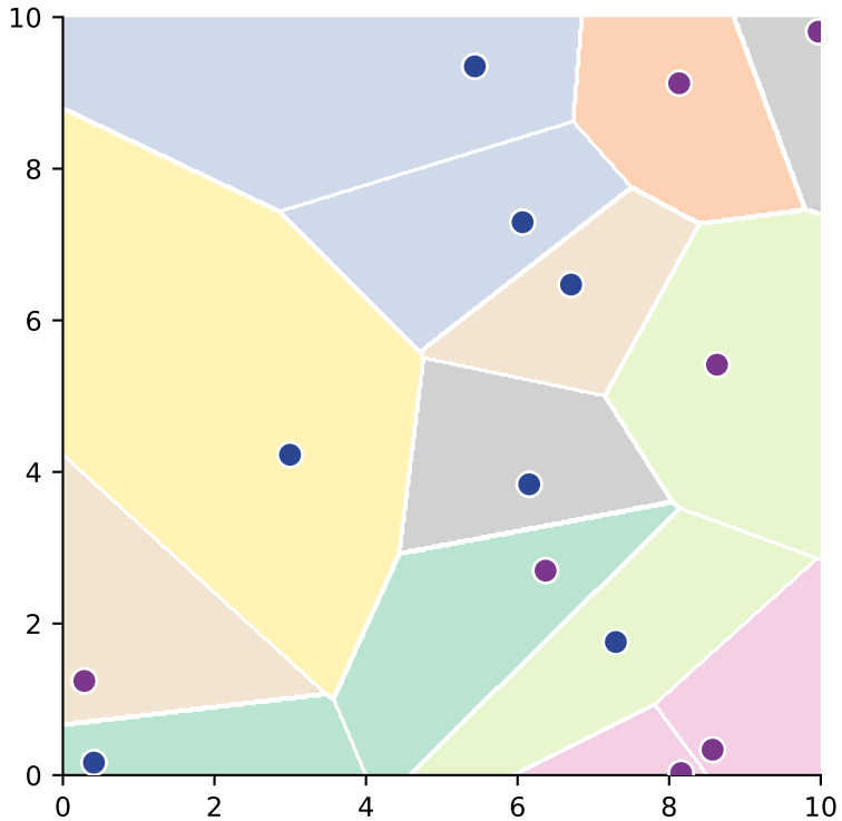
one cell per training point: the Voronoi tessellation
