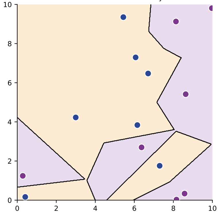
merge cells with the same label: the 1-NN decision boundary
