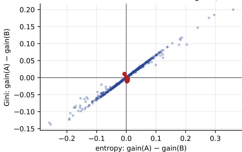
1197 random 2-attribute contests: 1191 agree (99.50%)
