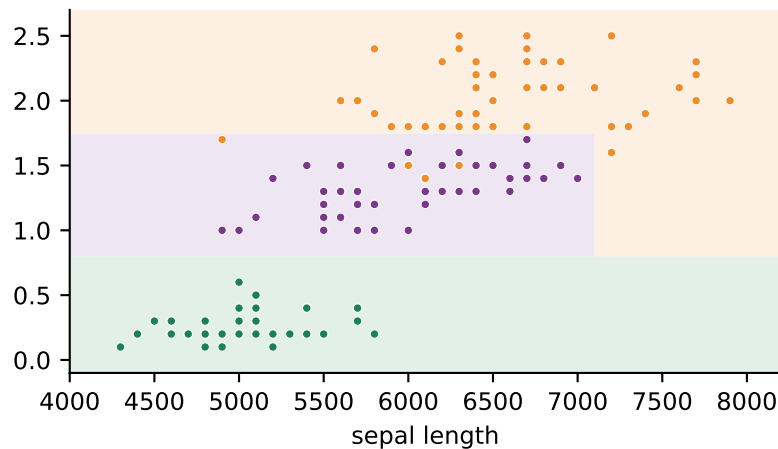
5-nearest neighbours, sepal length x1000 5-fold accuracy 0.7933
