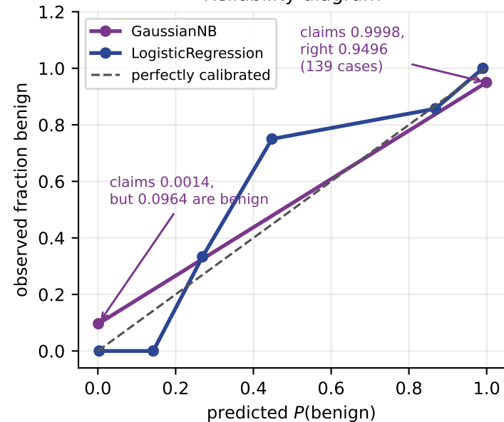
Reliability diagram
