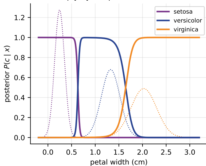
Multiply by the prior, then normalise
