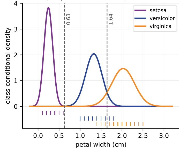
p(x | c) : one Gaussian per class
