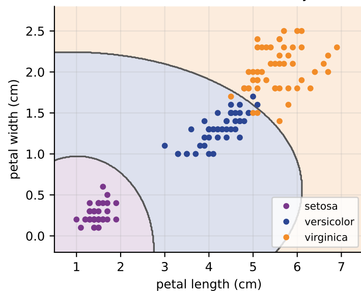
Two features, resubstitution accuracy 0.9600
