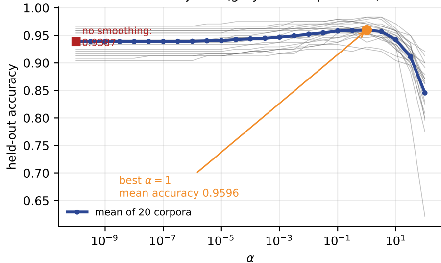
MultinomialNB, 20 corpora of 600 documents of 40 words, vocabulary 300 (grey: one corpus each)
