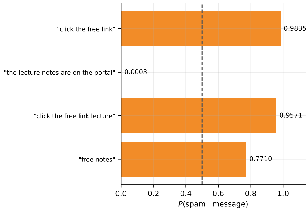
MultinomialNB, \alpha = 1
