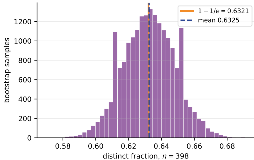
20 000 bootstrap samples of the training split
