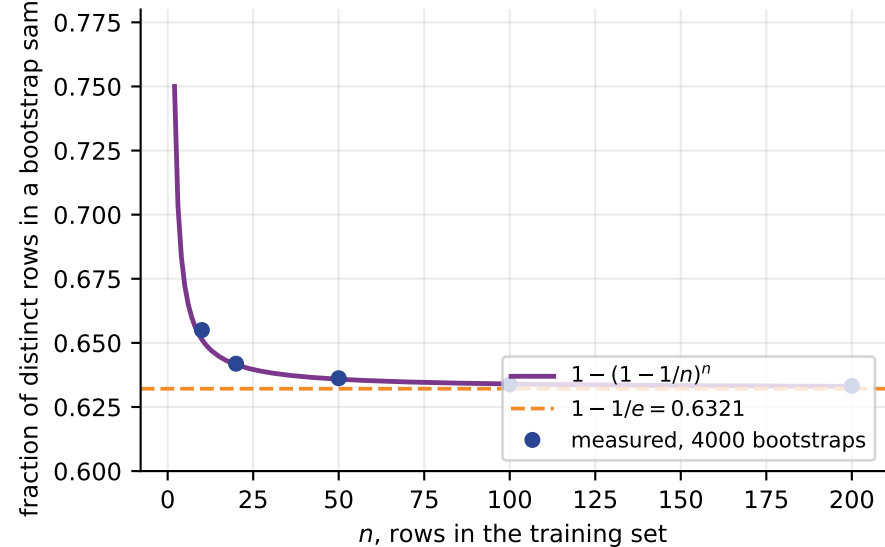
Each bag holds about 63.2% of the rows
