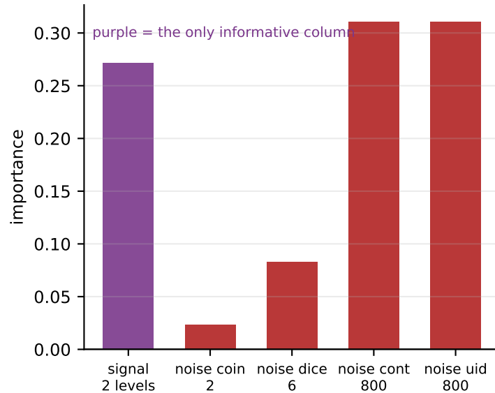
Impurity importance ranks two useless columns first
