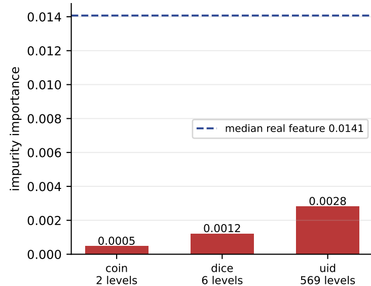
breast_cancer: three planted columns, all of them pure noise
