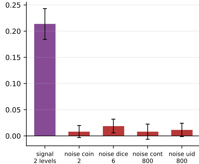
Permutation importance gets the ordering right
