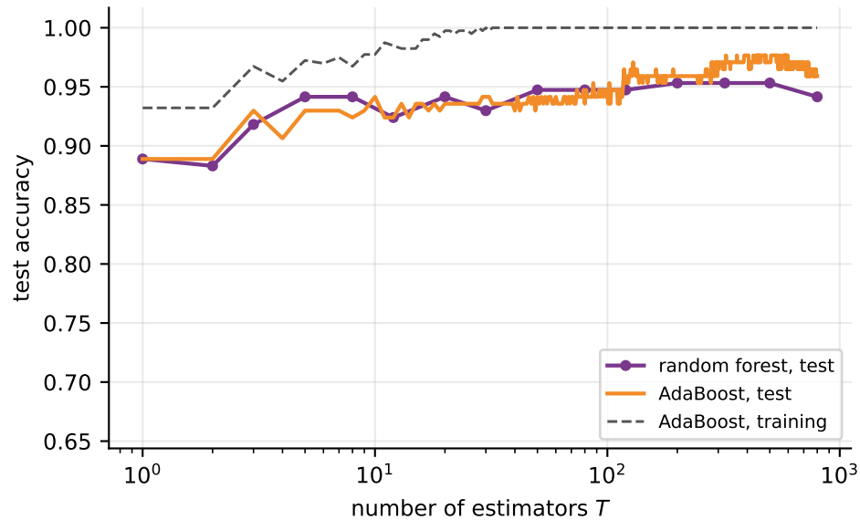
clean labels
