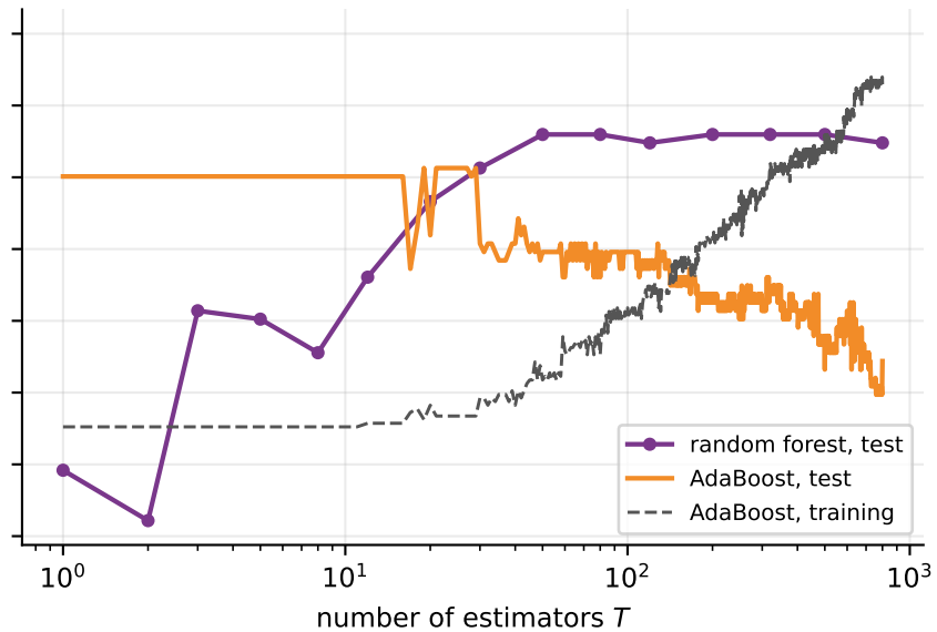
25% of training labels flipped
